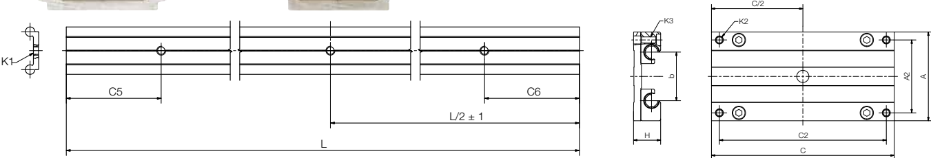
drylin® W special rails with 3 holes, 3/8" thread Dimensions [mm]
